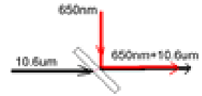
Beam combiner
